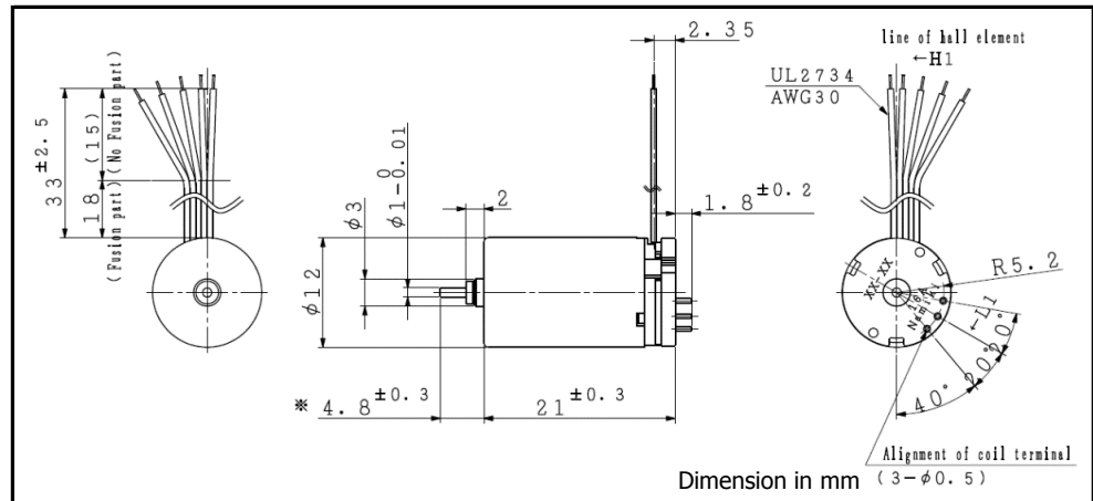
For combination with gearhead: SSG12, SPG12
